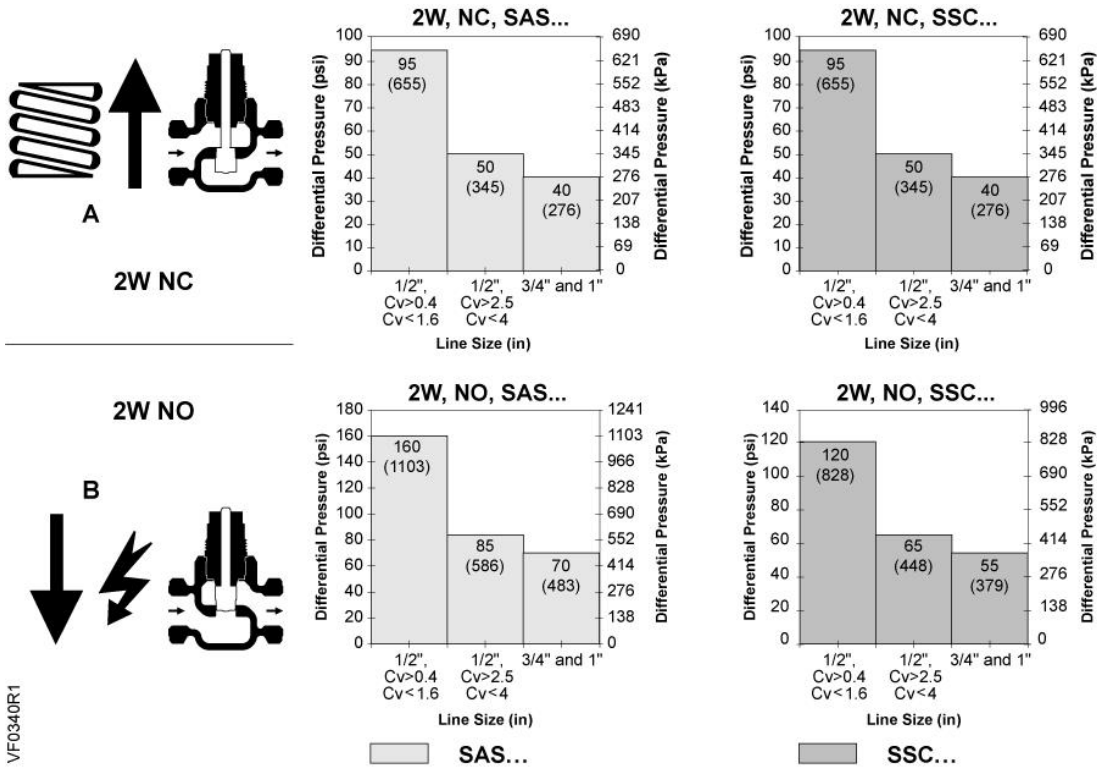
Figure 2. Close-off Pressures.
